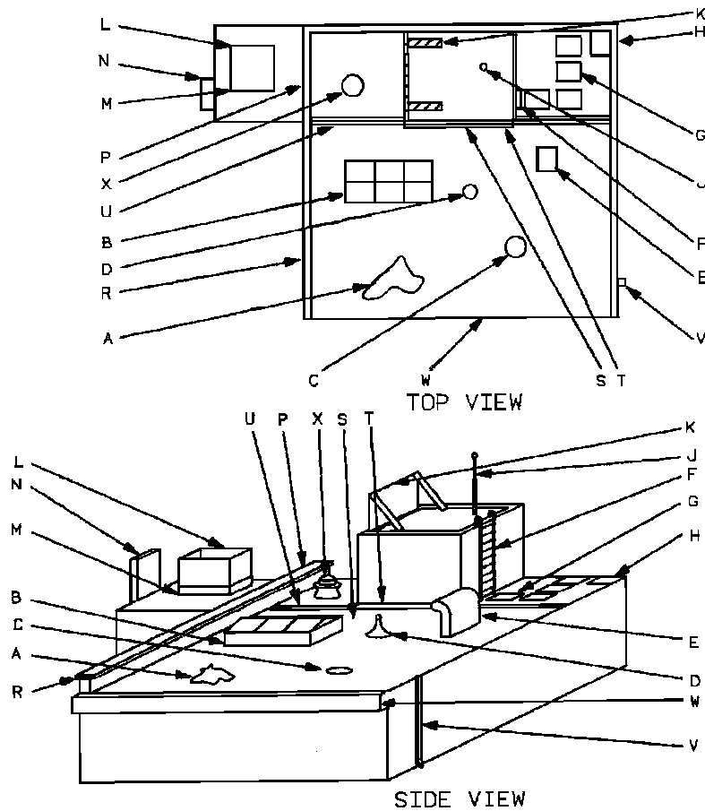
SAMPLE SKETCHED ROOF PLAN
